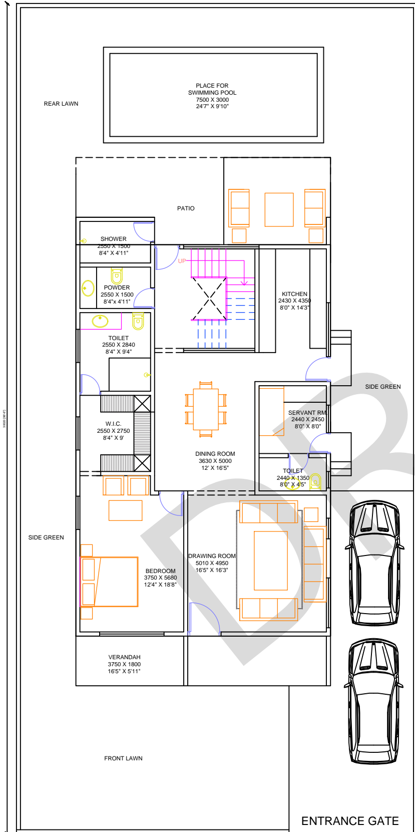
GROUND FLOOR
